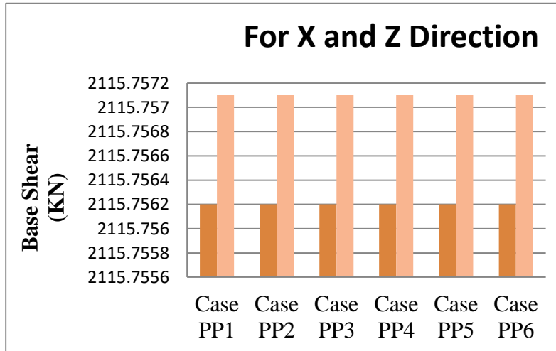
Figure 3: Base shear for soft Soil
