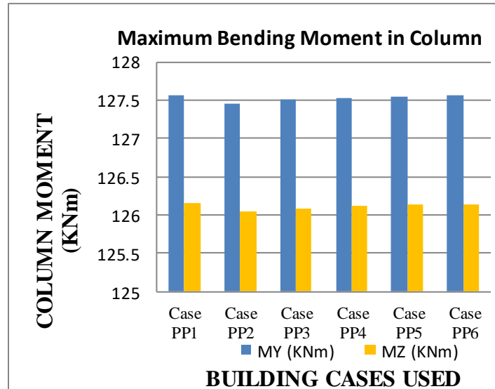
Figure 6: Bending Moment in column in soft soil
