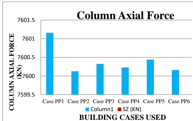
Figure 4: Axial Force in column in soft soil
