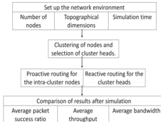
Figure 2. Flow process of the proposed model
